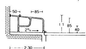
5 Lying boxes for cows
